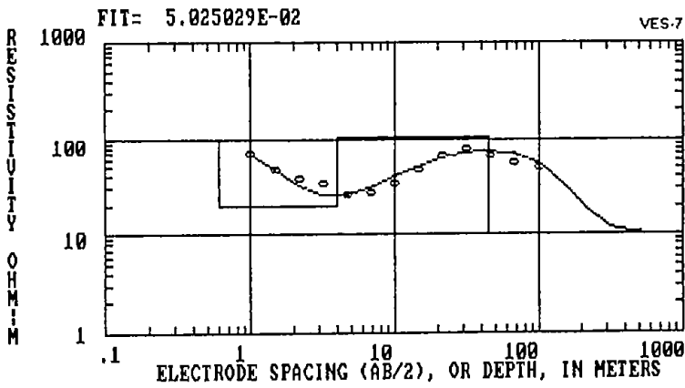
Fig.4.9 a) Field Curve b) Automatic Interpreted Results c) Reduced Multilayer Model of VES-7
