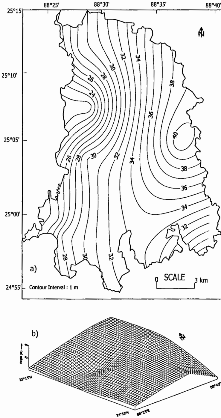
Fig.- 2.2: Contour Map showing the Surface Configuration of the Area. a) Contour Map; b) Trend
