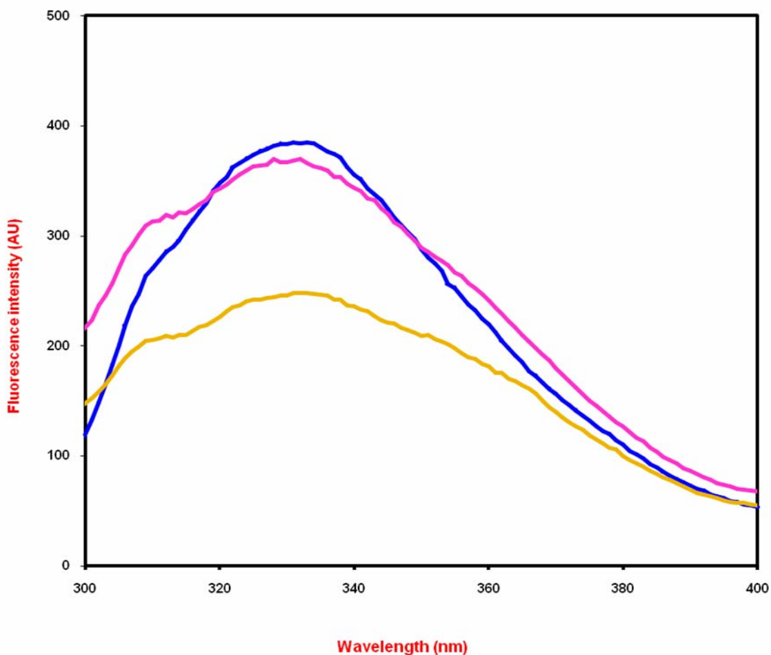
Figure 3.4 Fluorescence emission spectra of 50 \mu\text{g/ml} NNTL in presence of O -nitrophenyl- \beta -D-galactopyranoside.
