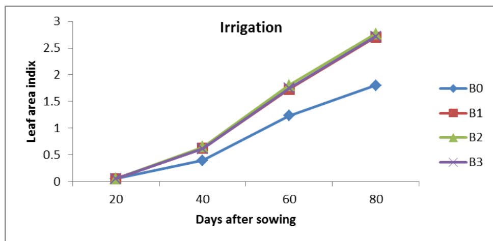
Figure 6. Effect of irrigation, sulphur and boron of leaf area index at different days after sowing (DAS) in 2013-2014
