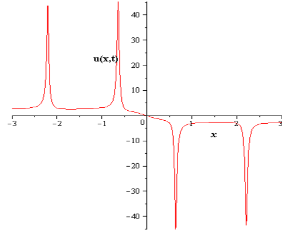
Fig-2.2: Kinky-periodic wave solution for a_4 = 1, b_1 = 0, b_2 = b_3 = w_2 = k_2 = 2, k_1 = 3 of the propagation pattern. Fig-2.2(a): 2D plot along t = 0 shows the wave propagation pattern.
