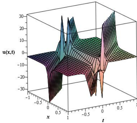
Fig-2.2: Kinky-periodic wave solution for a_4 = 1, b_1 = 0, b_2 = b_3 = w_2 = k_2 = 2, k_1 = 3 of the propagation pattern. Fig-2.2(a): 2D plot along t = 0 shows the wave propagation pattern.
