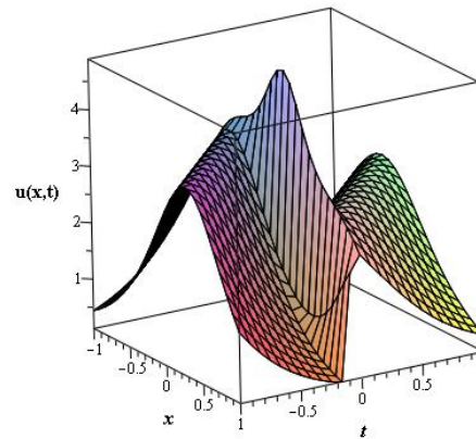
Fig-2.4: Collision of two kink with a bell shaped soliton solution for b_2 = b_3 = w_2 = k_2 = 2, a_4 = 1, b_1 = 0, k_1 = 3 of the real part of u_{27,28} .
