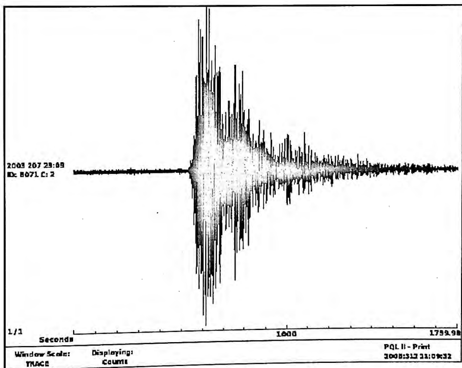
Fig. 3.4 North-South Ground accelerated seismic wave recorded at Dhaka University of M 5.6 earthquake on 26 July 2003 of 23:18:17 UTC time that occurred at the south-west of Daluchari, Chittagong.
