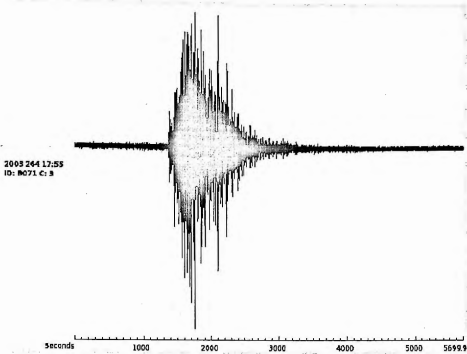
Fig. 3.11 East-West Ground accelerated seismic wave recorded at Dhaka University of M 6.6 earthquake on 21 September 2003 of 18:16:13 UTC time that occurred at the south of Meiktila, Myanmar.
