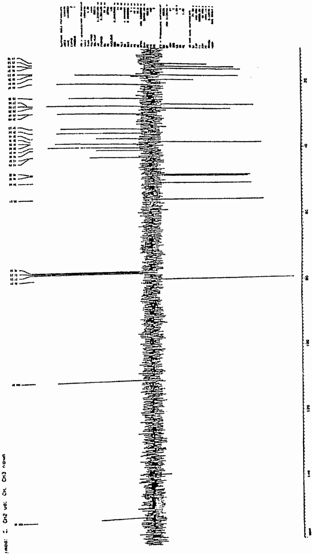
Figure-5.8: ^{13}\text{C-NMR} spectrum of compound CBC-3
